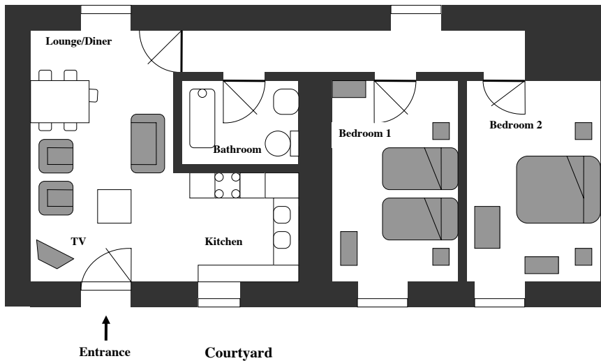
FARMHOUSE APARTMENT 2 Ground Floor
